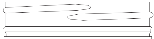
100mm Multi-Start Screw Neck
