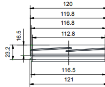
Screw Neck
